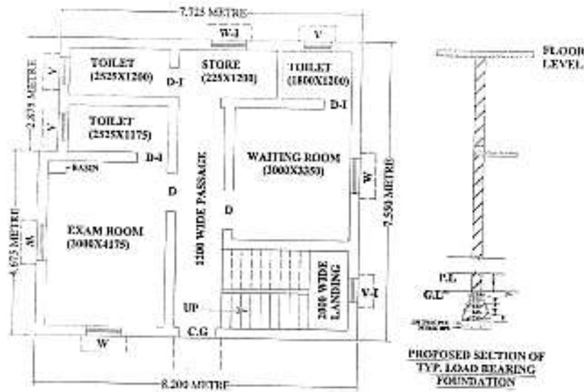
PROPOSED ARCHITECTURAL PLAN OF SUB-CENTRE GROUND FLOOR
